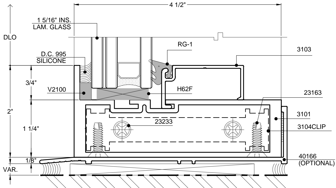
12 TYPICAL SILL
